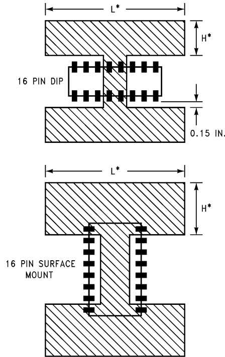
FIGURE 2. Copper Heatsink Patterns
