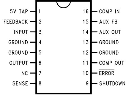
16-Pin DIP
